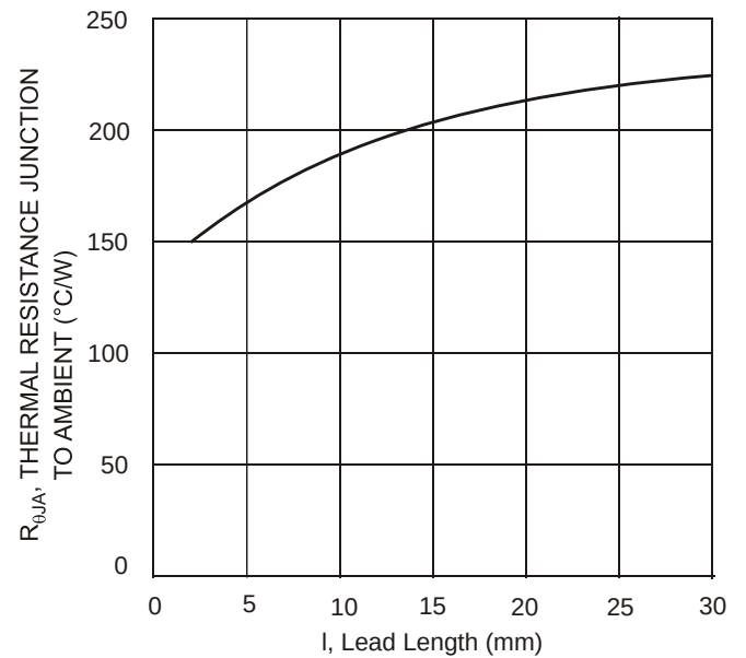
Fig. 2 Typical Thermal Resistance vs. Lead Length
